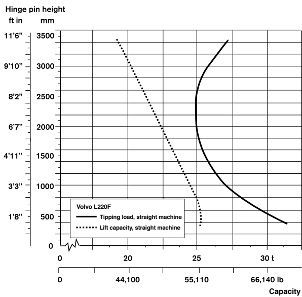
Volvo L220F*
