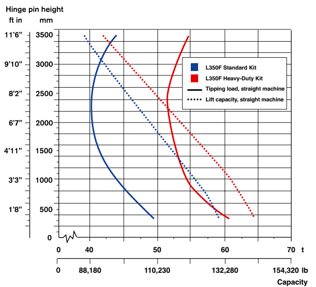
Volvo L350F**
